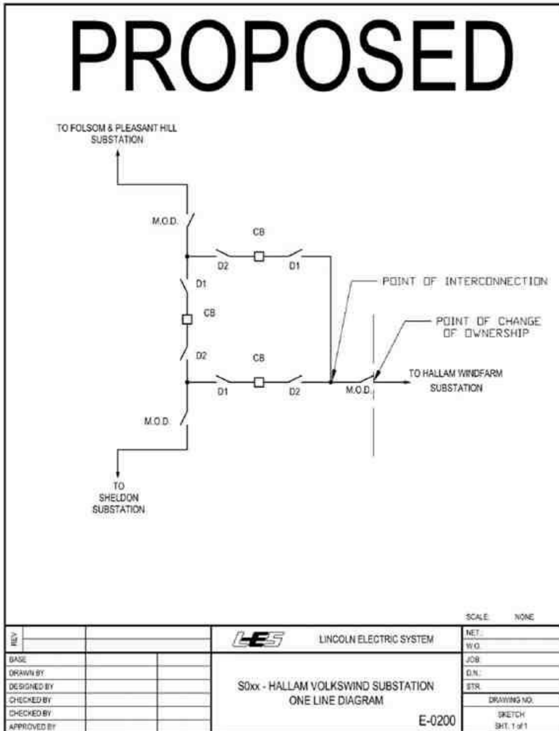
Figure A1 – One-line diagram of the Point of Interconnection
